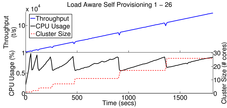
Figure 4.10: Elastic Management - Load-Aware Provisioning.
