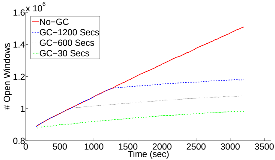
Figure 5.13: Garbage Collection evaluation
