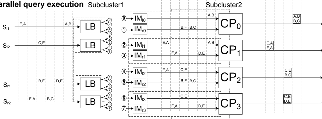
Figure 3.5: Cartesian Product Sample Execution
