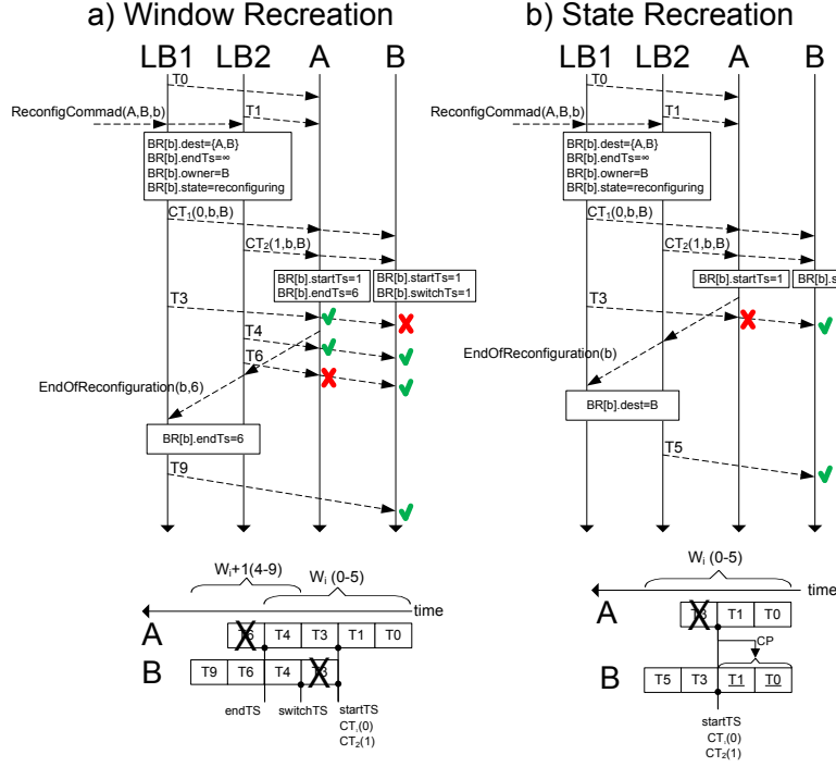
Figure 4.5: Sample reconfigurations.
