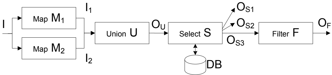
Figure 7.3: Blacklist Query
