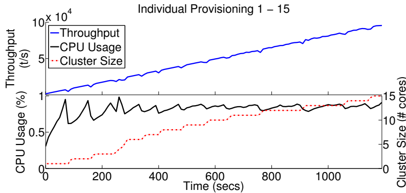
Figure 4.9: Elastic Management - Individual Provisioning.
