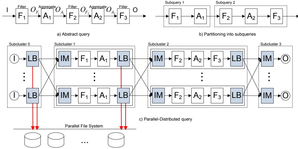
Figure 5.7: Linear Road.
