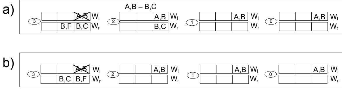
Figure 3.6: Cartesian Product Sample Execution
